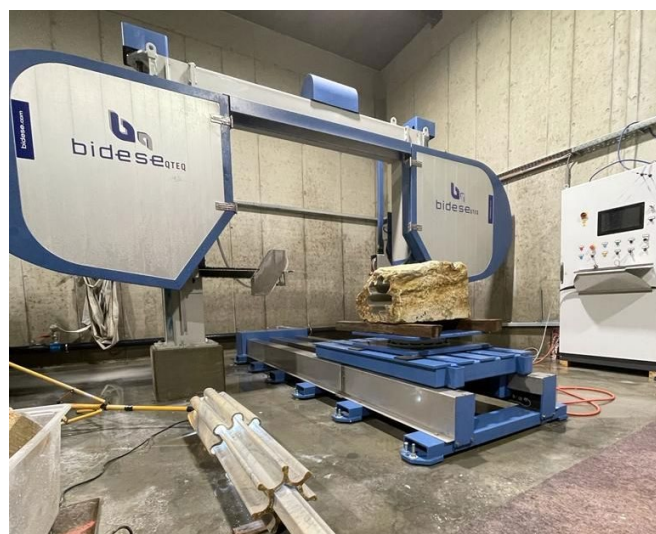
MONOFIOS a CNC 3 a 5x
